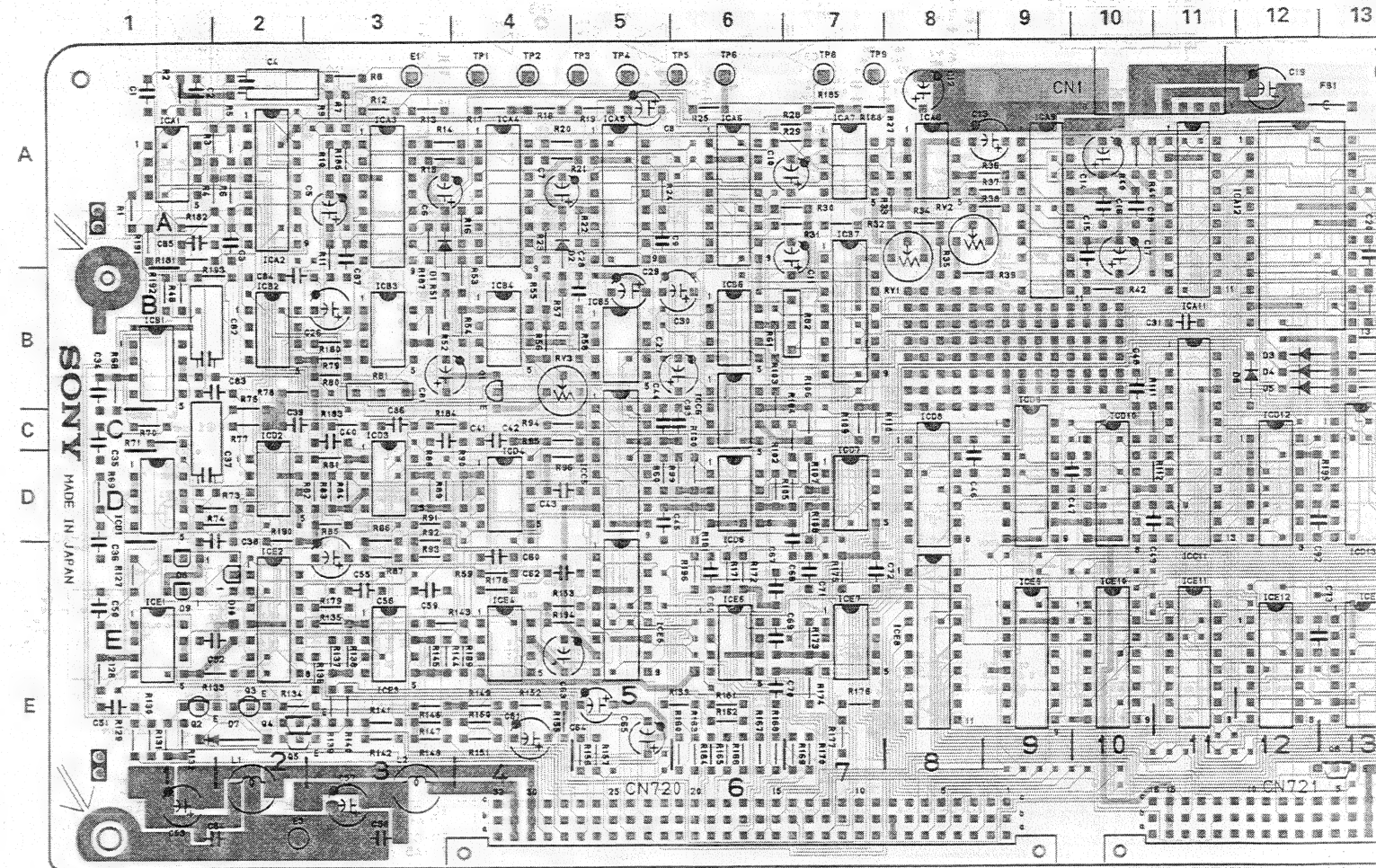
1-620-885-13 COMPONENT SIDE
